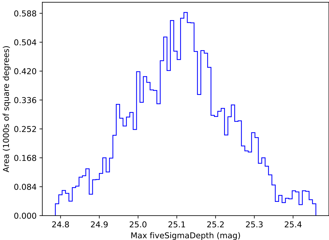
noroll_mjdp60_v3.4_10yrs WFD g band: Max fiveSigmaDepth
