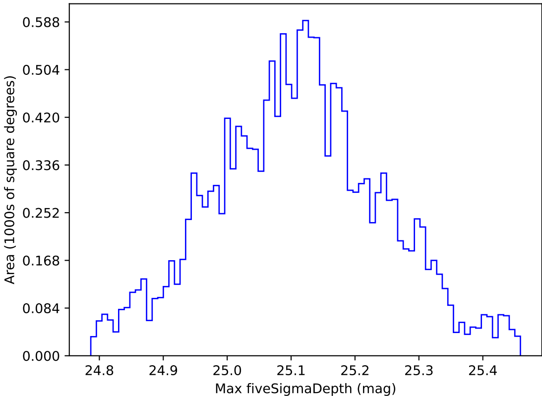
noroll_mjdp60_v3.4_10yrs WFD all bands: Max fiveSigmaDepth
