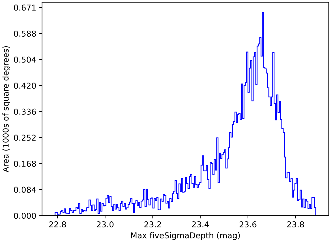
noroll_mjdp60_v3.4_10yrs All sky z band: Max fiveSigmaDepth
