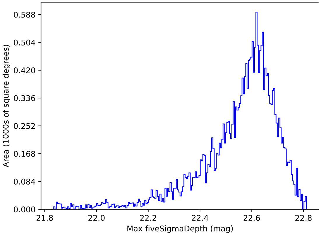
noroll_mjdp60_v3.4_10yrs All sky y band: Max fiveSigmaDepth
