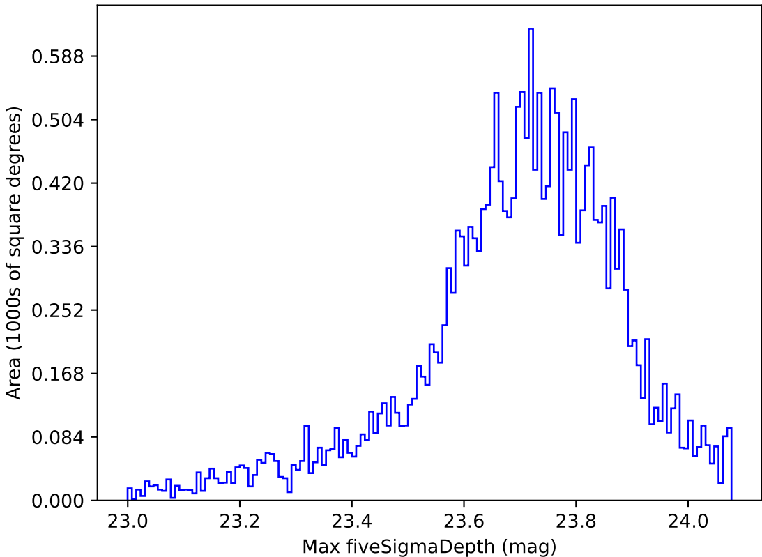
noroll_mjdp60_v3.4_10yrs All sky u band: Max fiveSigmaDepth
