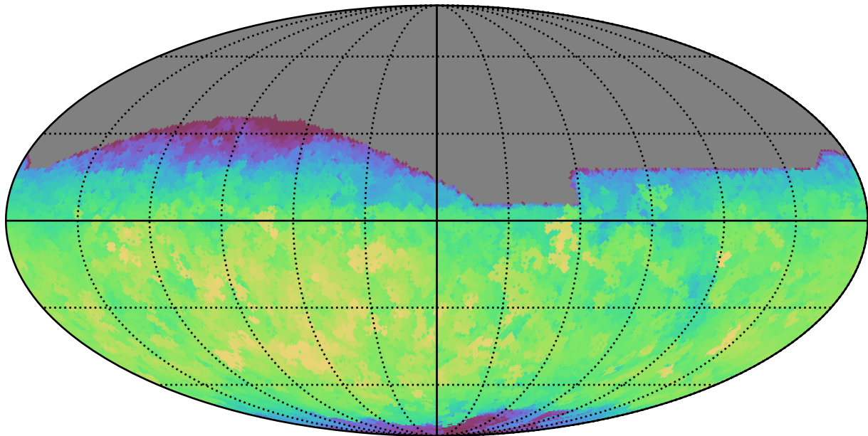
noroll_mjdp60_v3.4_10yrs All sky r band: Max fiveSigmaDepth
