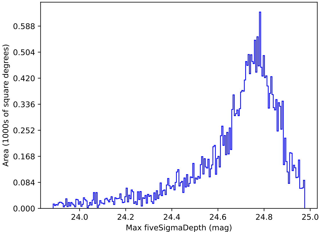
noroll_mjdp60_v3.4_10yrs All sky r band: Max fiveSigmaDepth
