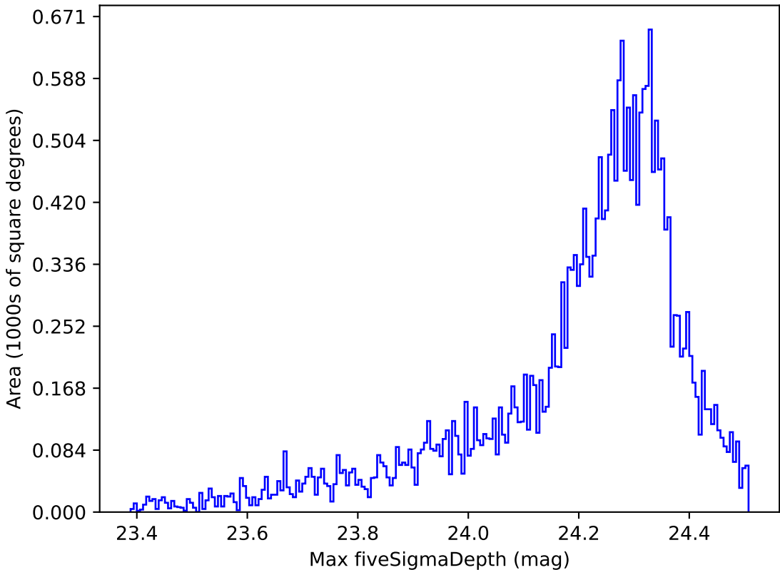
noroll_mjdp60_v3.4_10yrs All sky i band: Max fiveSigmaDepth
