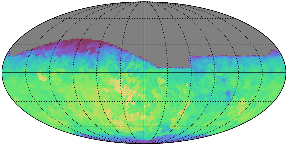
noroll_mjdp60_v3.4_10yrs All sky g band: Max fiveSigmaDepth
