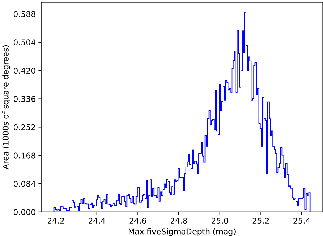
noroll_mjdp60_v3.4_10yrs All sky g band: Max fiveSigmaDepth
