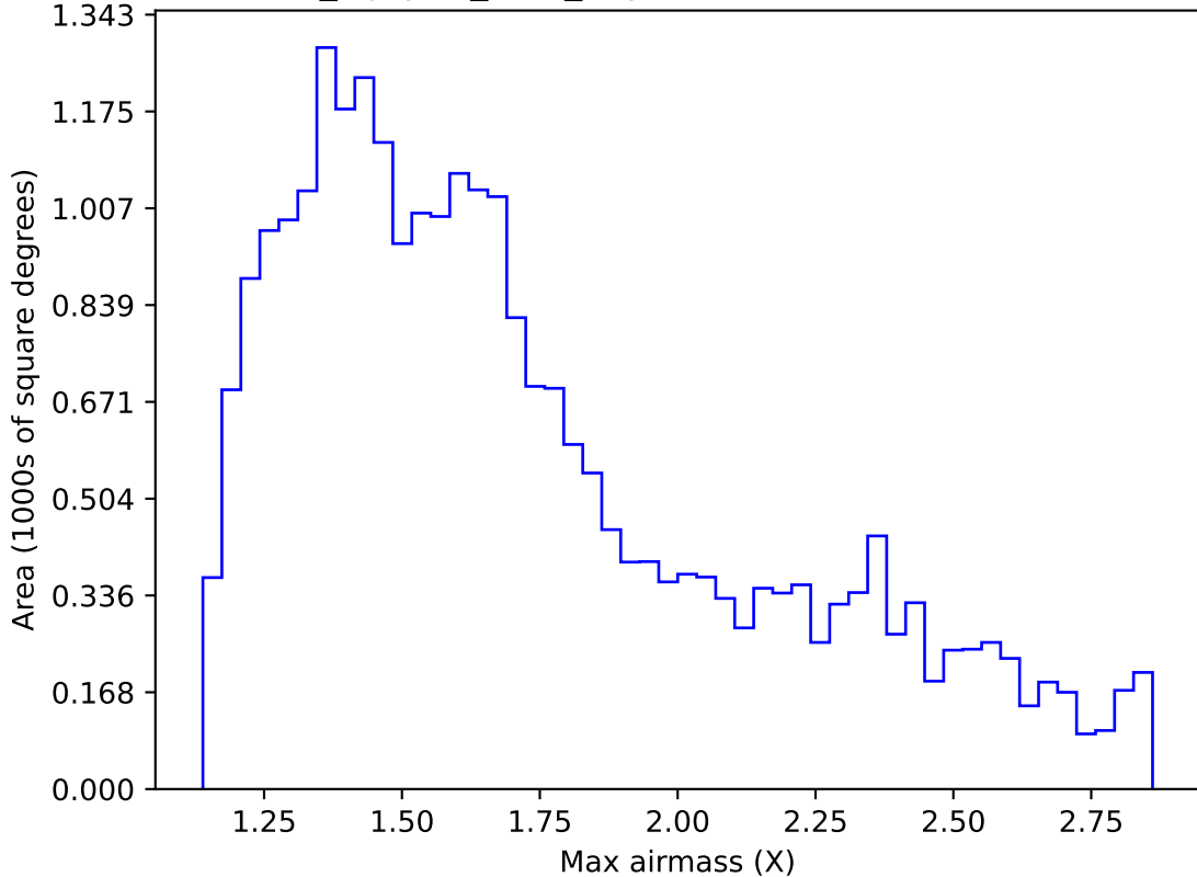
noroll_mjdp60_v3.4_10yrs Yr 1 z band: Max airmass
