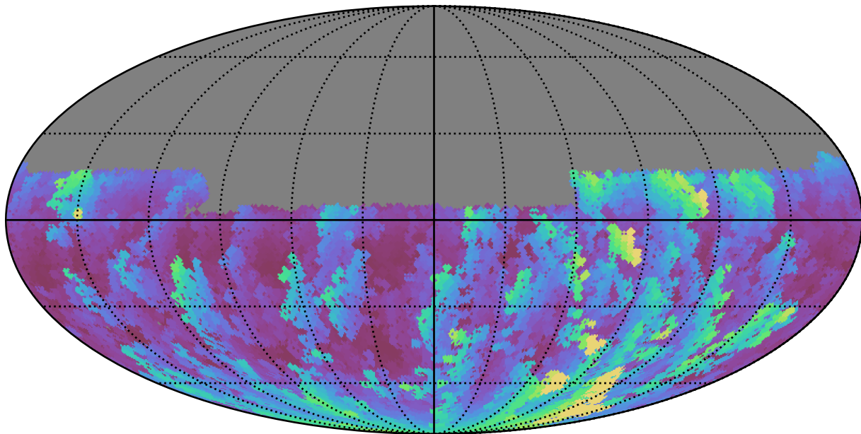
noroll_mjdp60_v3.4_10yrs Yr 1 u band: Max airmass
