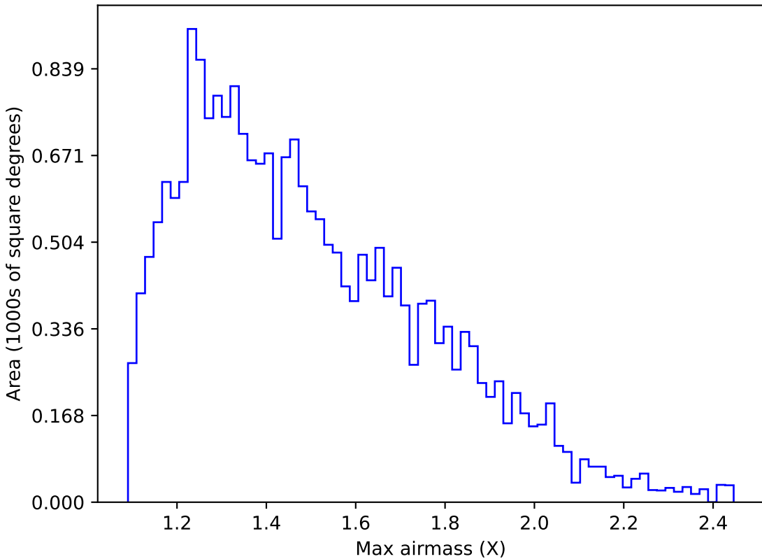
noroll_mjdp60_v3.4_10yrs Yr 1 u band: Max airmass
