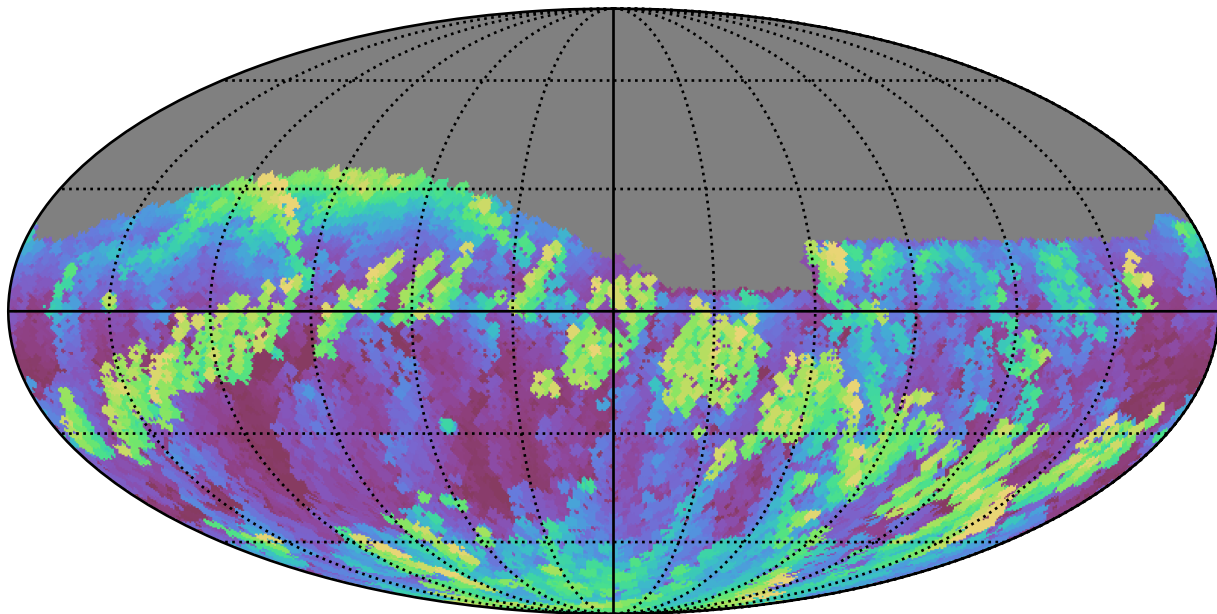
noroll_mjdp60_v3.4_10yrs Yr 1 r band: Max airmass
