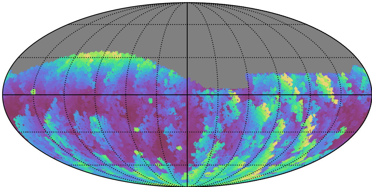
noroll_mjdp60_v3.4_10yrs Yr 1 g band: Max airmass
