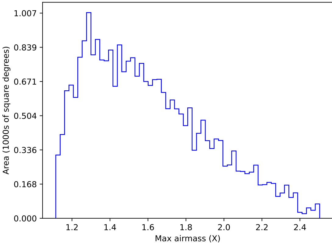
noroll_mjdp60_v3.4_10yrs Yr 1 g band: Max airmass
