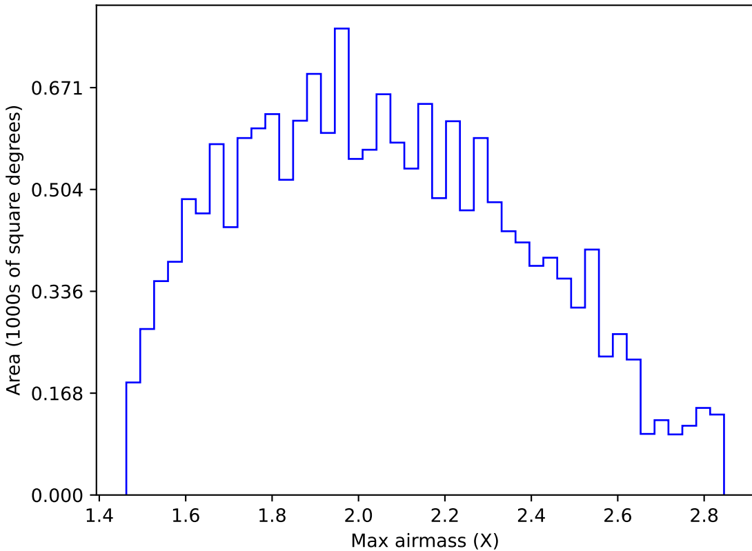
noroll_mjdp60_v3.4_10yrs WFD y band: Max airmass
