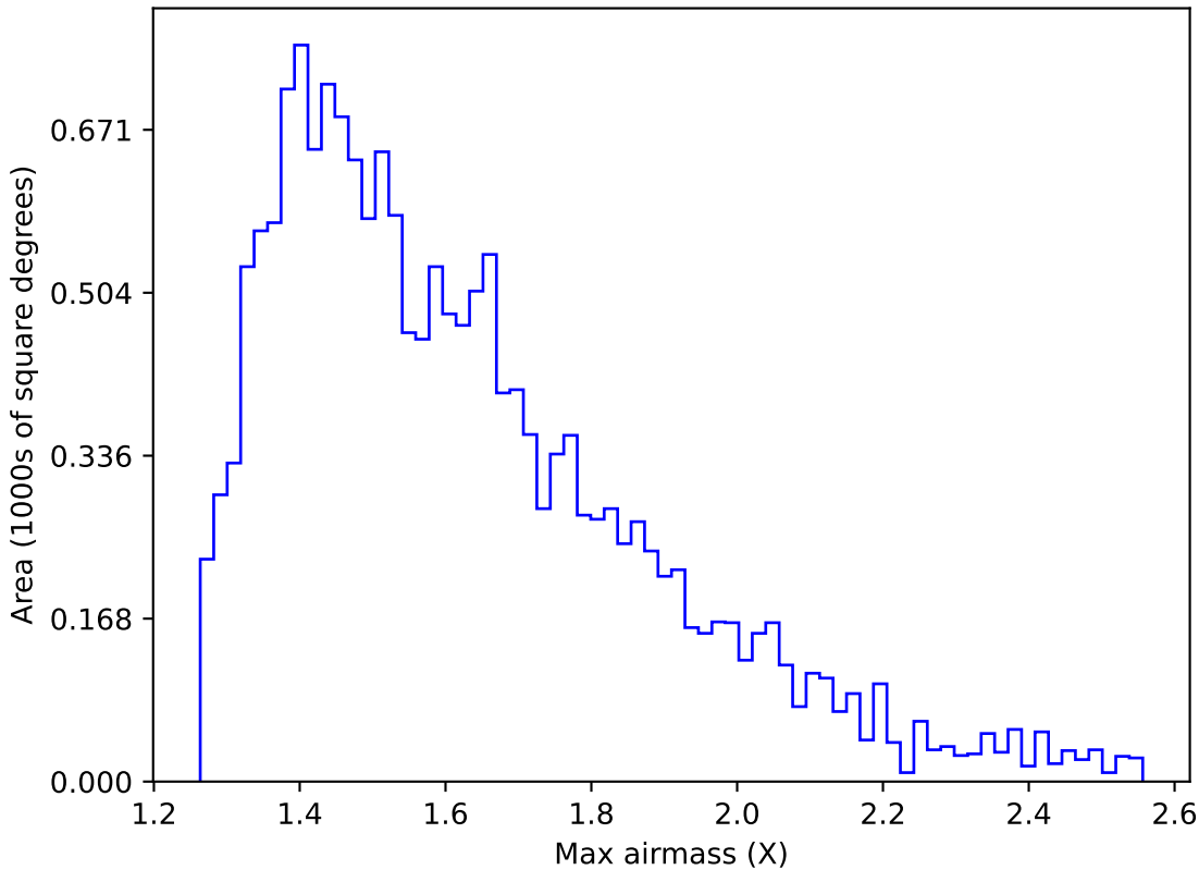
noroll_mjdp60_v3.4_10yrs WFD u band: Max airmass
