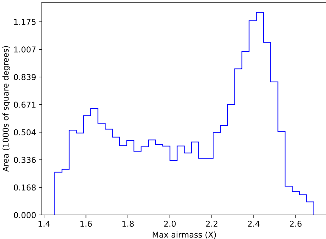
noroll_mjdp60_v3.4_10yrs WFD r band: Max airmass
