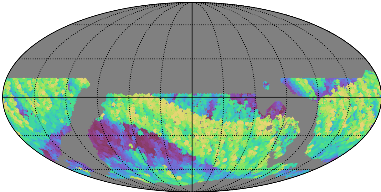
noroll_mjdp60_v3.4_10yrs WFD i band: Max airmass
