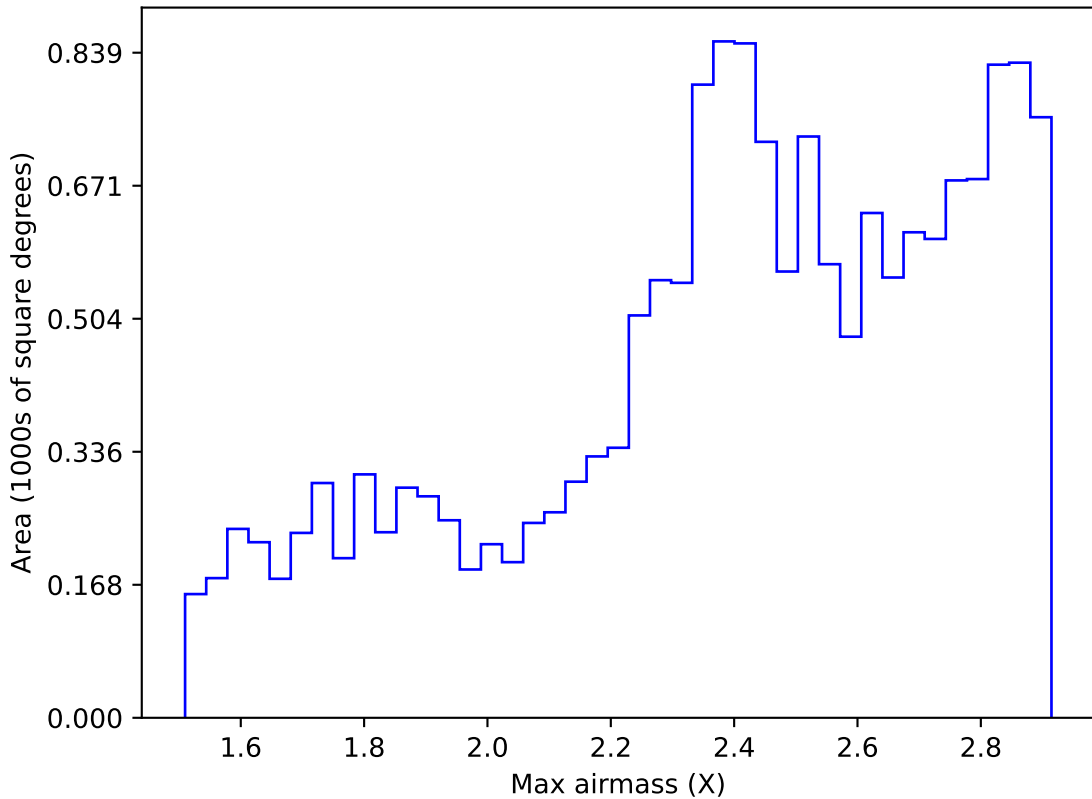
noroll_mjdp60_v3.4_10yrs WFD i band: Max airmass
