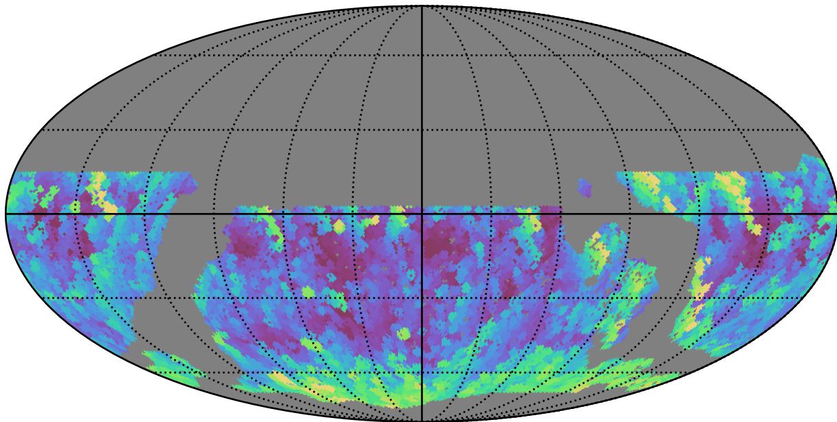
noroll_mjdp60_v3.4_10yrs WFD g band: Max airmass
