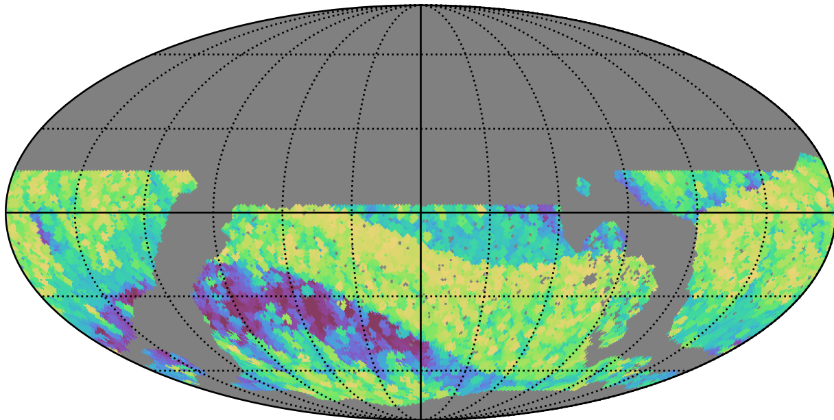
noroll_mjdp60_v3.4_10yrs WFD all bands: Max airmass
