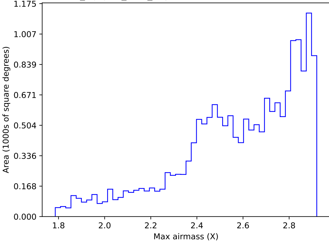
noroll_mjdp60_v3.4_10yrs WFD all bands: Max airmass
