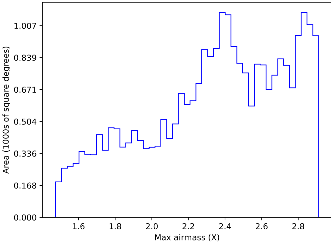
noroll_mjdp60_v3.4_10yrs All sky z band: Max airmass
