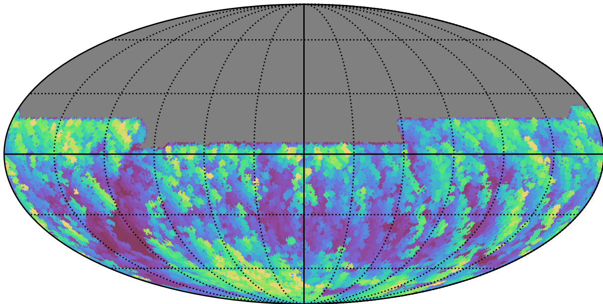
noroll_mjdp60_v3.4_10yrs All sky y band: Max airmass
