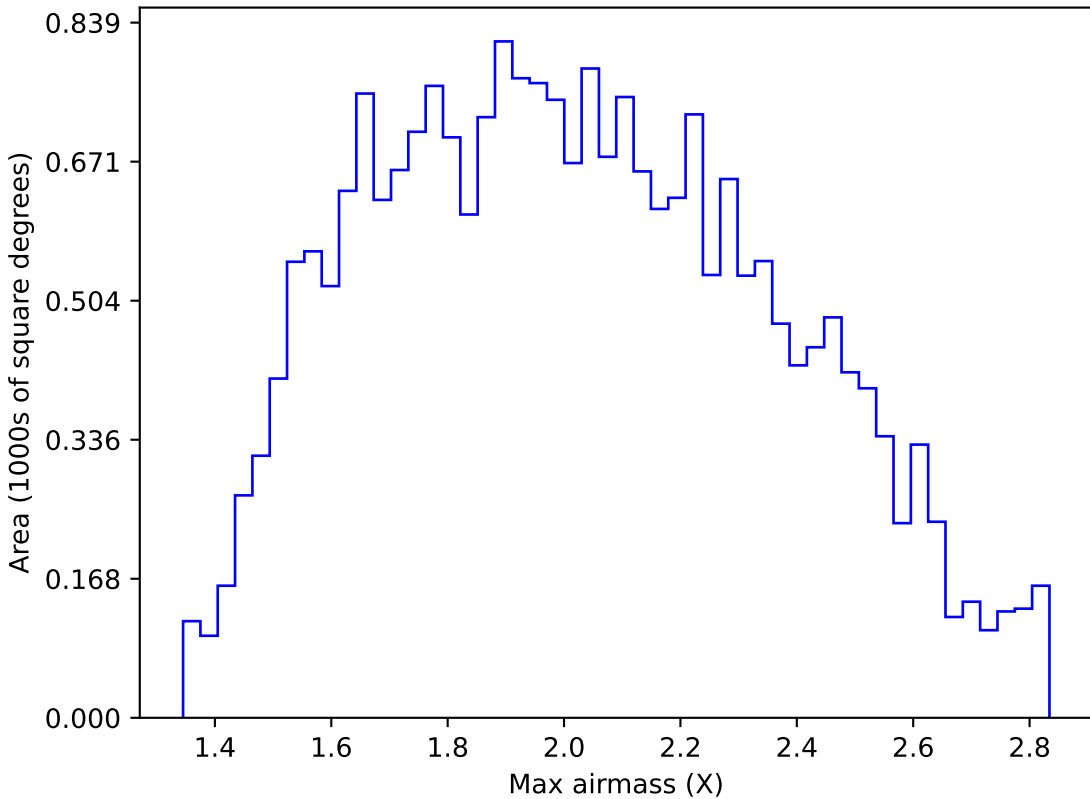
noroll_mjdp60_v3.4_10yrs All sky y band: Max airmass
