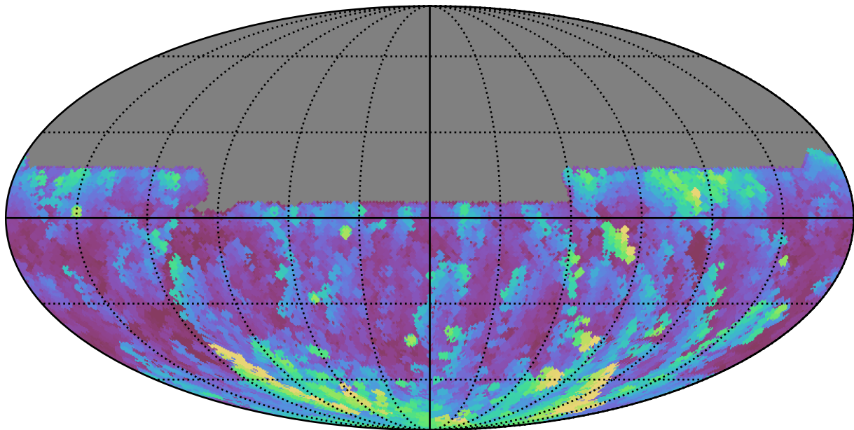
noroll_mjdp60_v3.4_10yrs All sky u band: Max airmass
