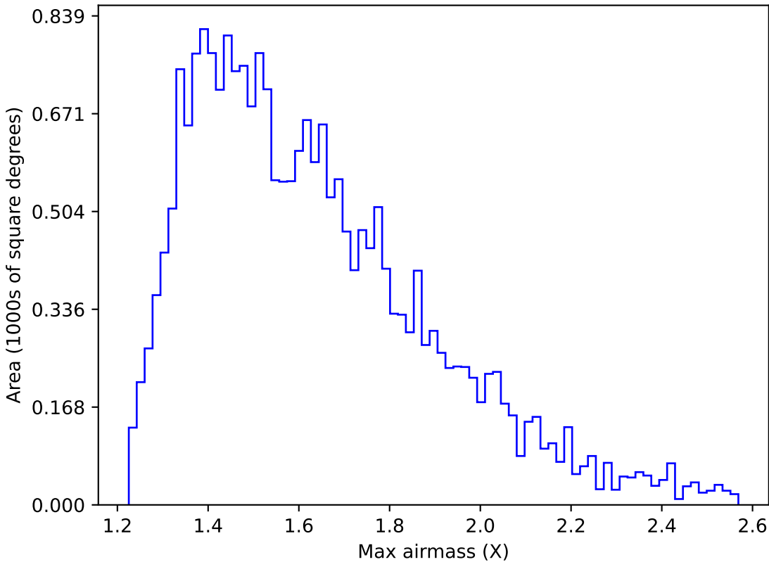
noroll_mjdp60_v3.4_10yrs All sky u band: Max airmass
