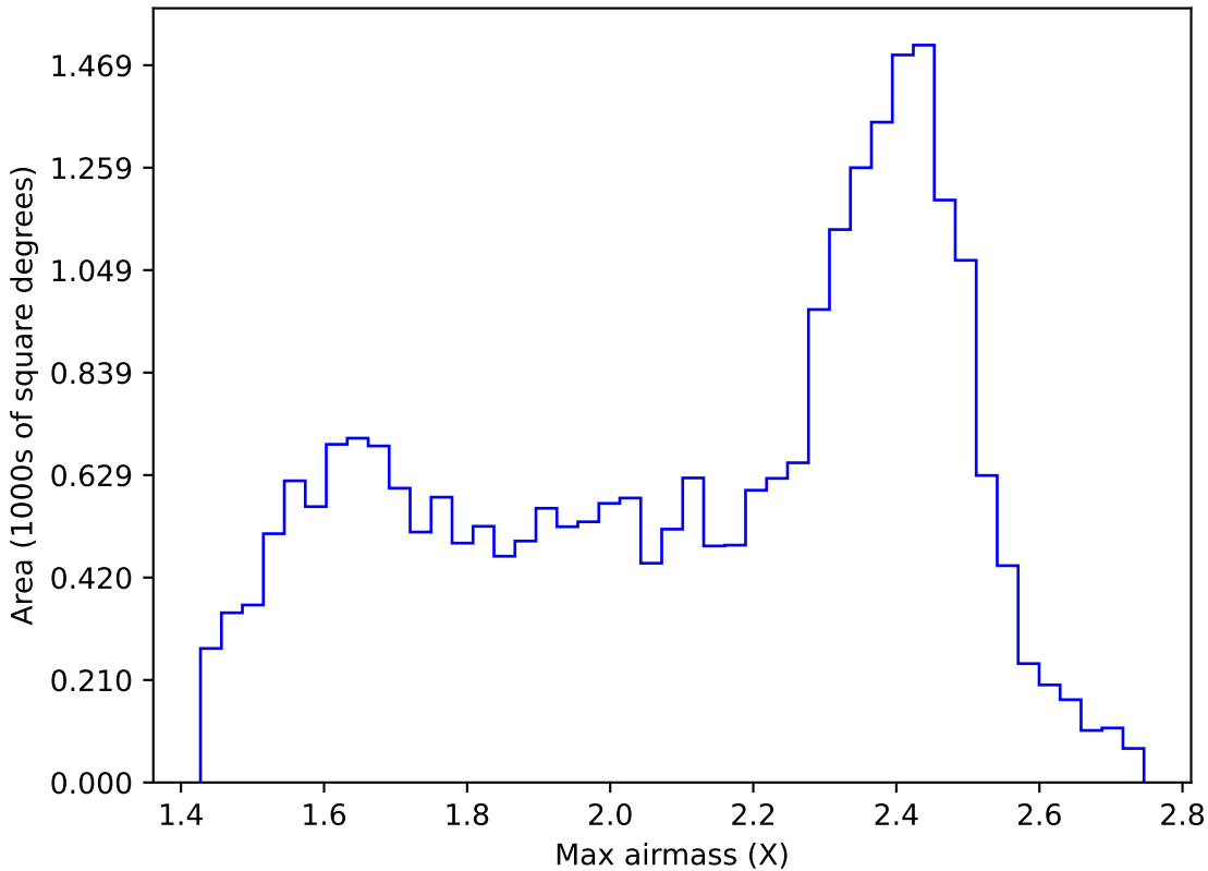
noroll_mjdp60_v3.4_10yrs All sky r band: Max airmass
