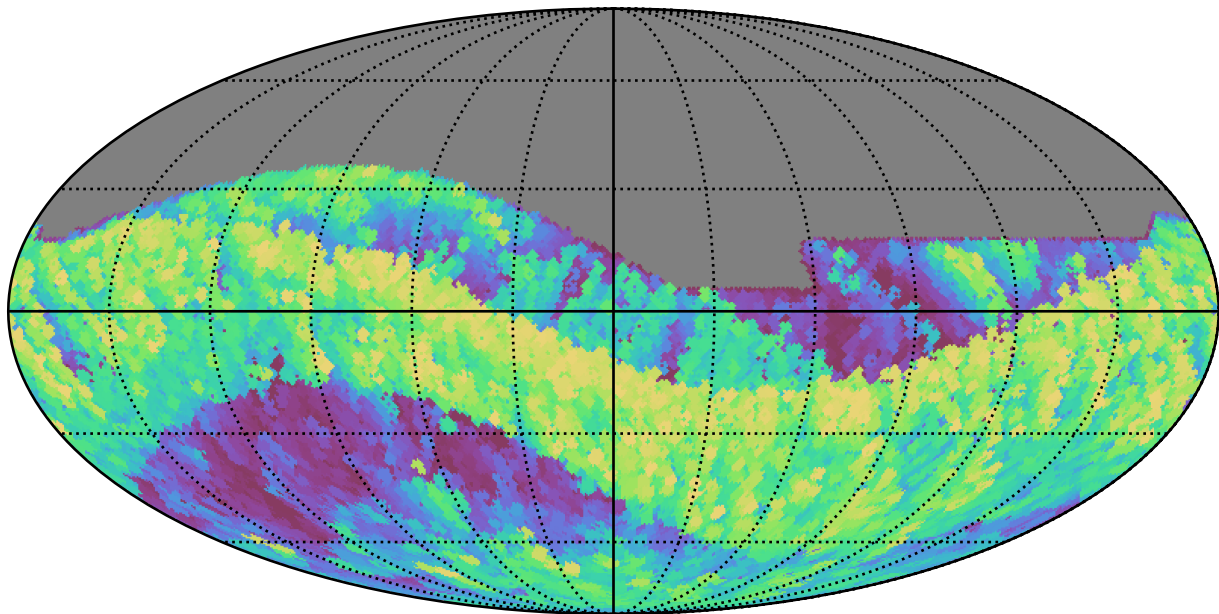
noroll_mjdp60_v3.4_10yrs All sky i band: Max airmass
