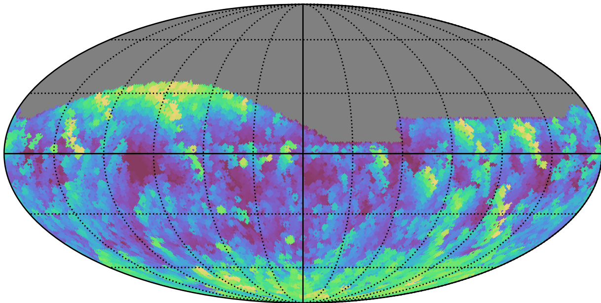
noroll_mjdp60_v3.4_10yrs All sky g band: Max airmass
