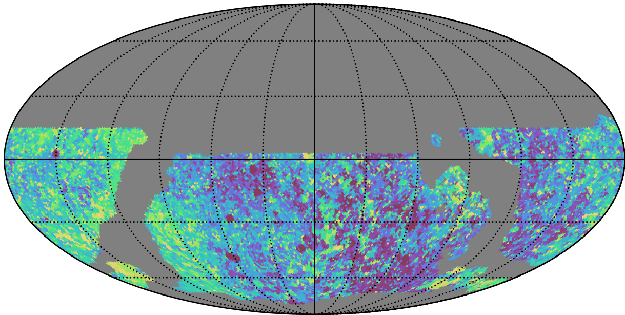
noroll_mjdp60_v3.4_10yrs WFD z band: Max Inter-Night Gap
