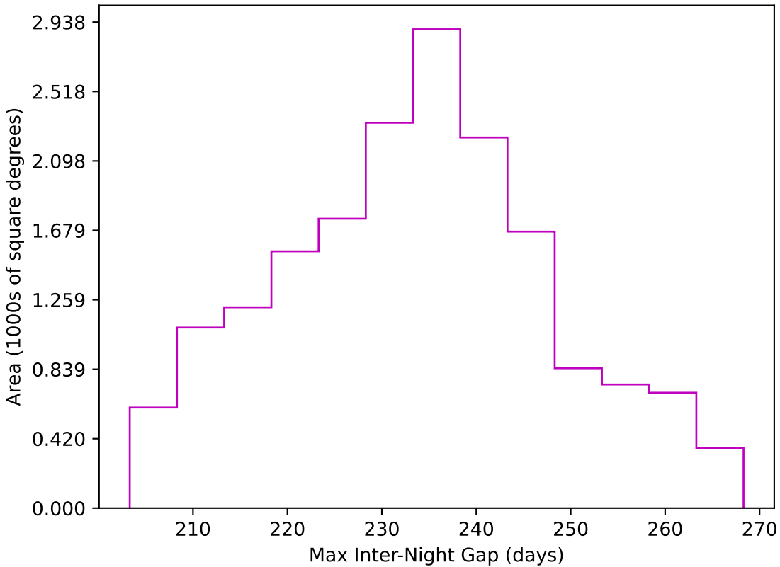
noroll_mjdp60_v3.4_10yrs WFD z band: Max Inter-Night Gap
