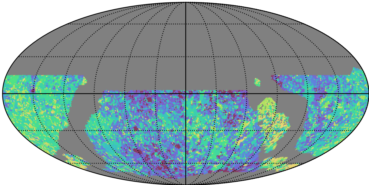
noroll_mjdp60_v3.4_10yrs WFD y band: Max Inter-Night Gap
