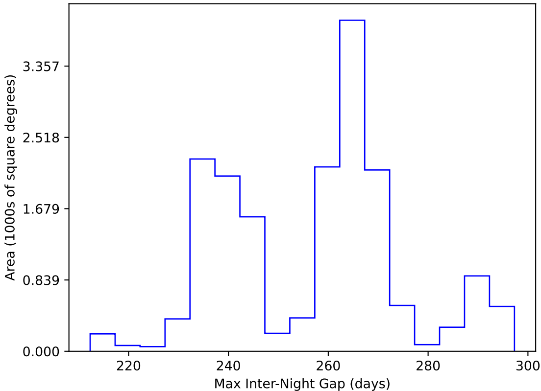
noroll_mjdp60_v3.4_10yrs WFD y band: Max Inter-Night Gap
