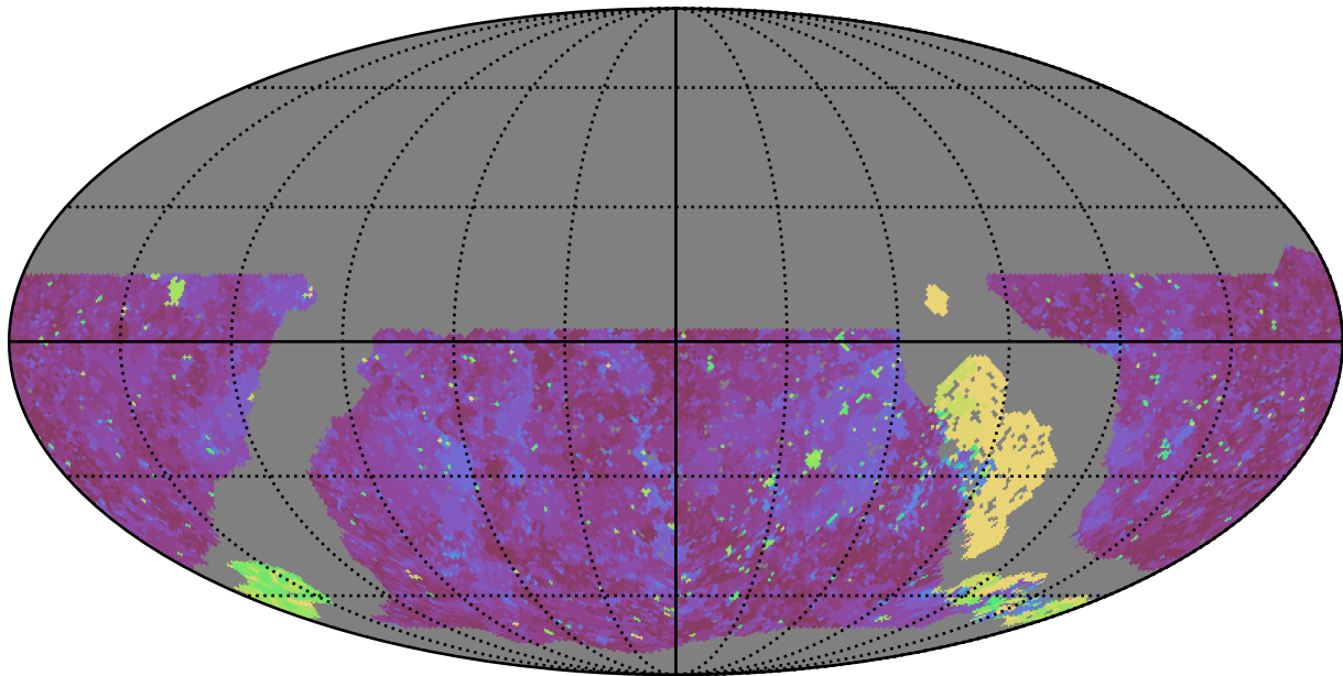
noroll_mjdp60_v3.4_10yrs WFD u band: Max Inter-Night Gap
