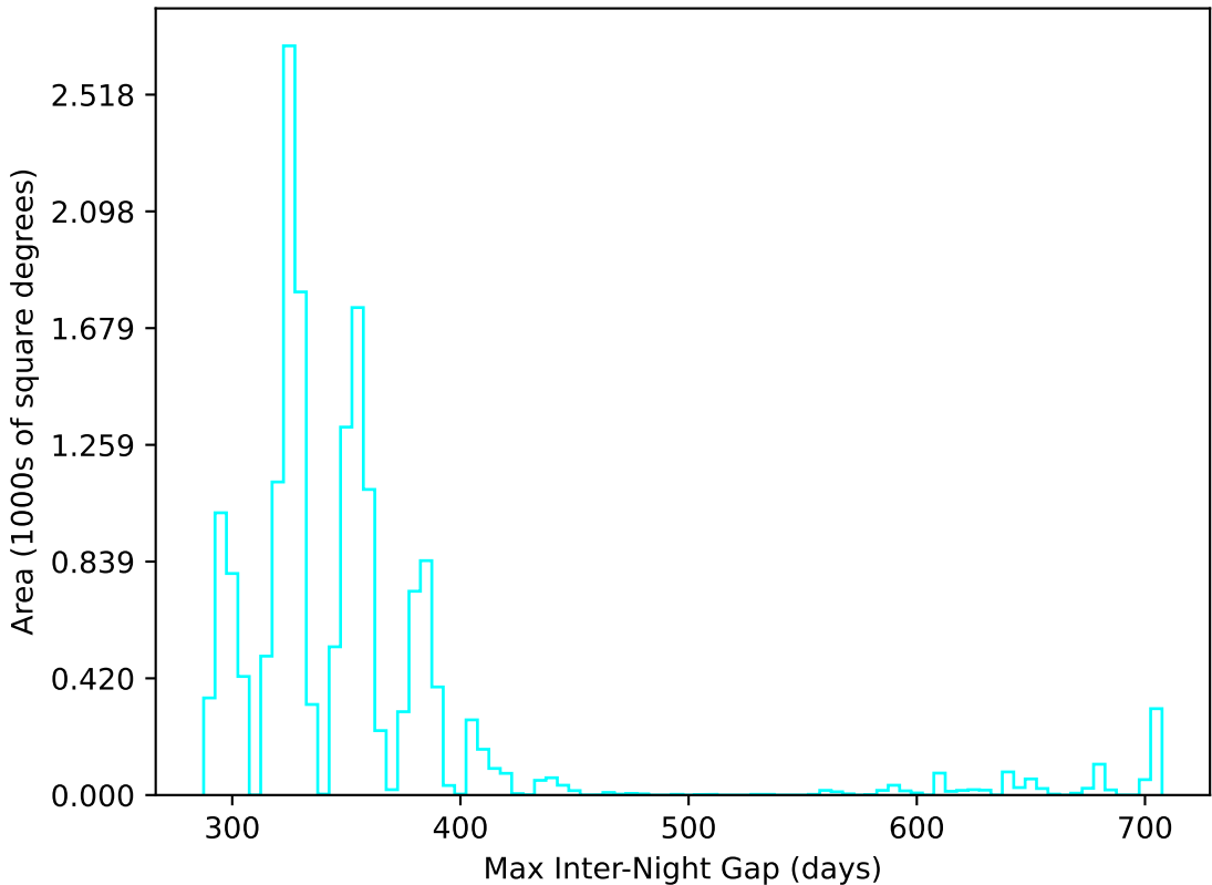
noroll_mjdp60_v3.4_10yrs WFD u band: Max Inter-Night Gap
