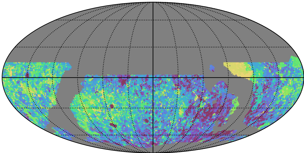
noroll_mjdp60_v3.4_10yrs WFD r band: Max Inter-Night Gap
