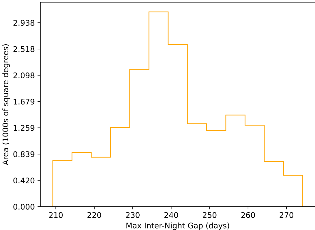
noroll_mjdp60_v3.4_10yrs WFD r band: Max Inter-Night Gap
