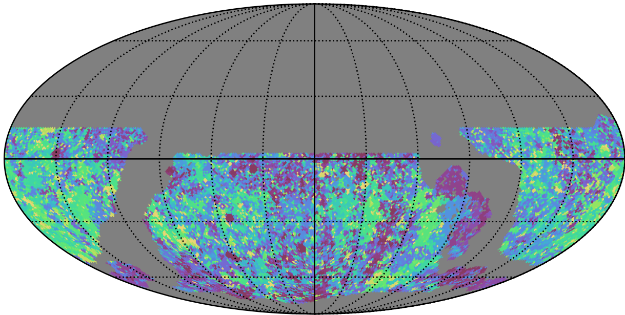
noroll_mjdp60_v3.4_10yrs WFD g band: Max Inter-Night Gap
