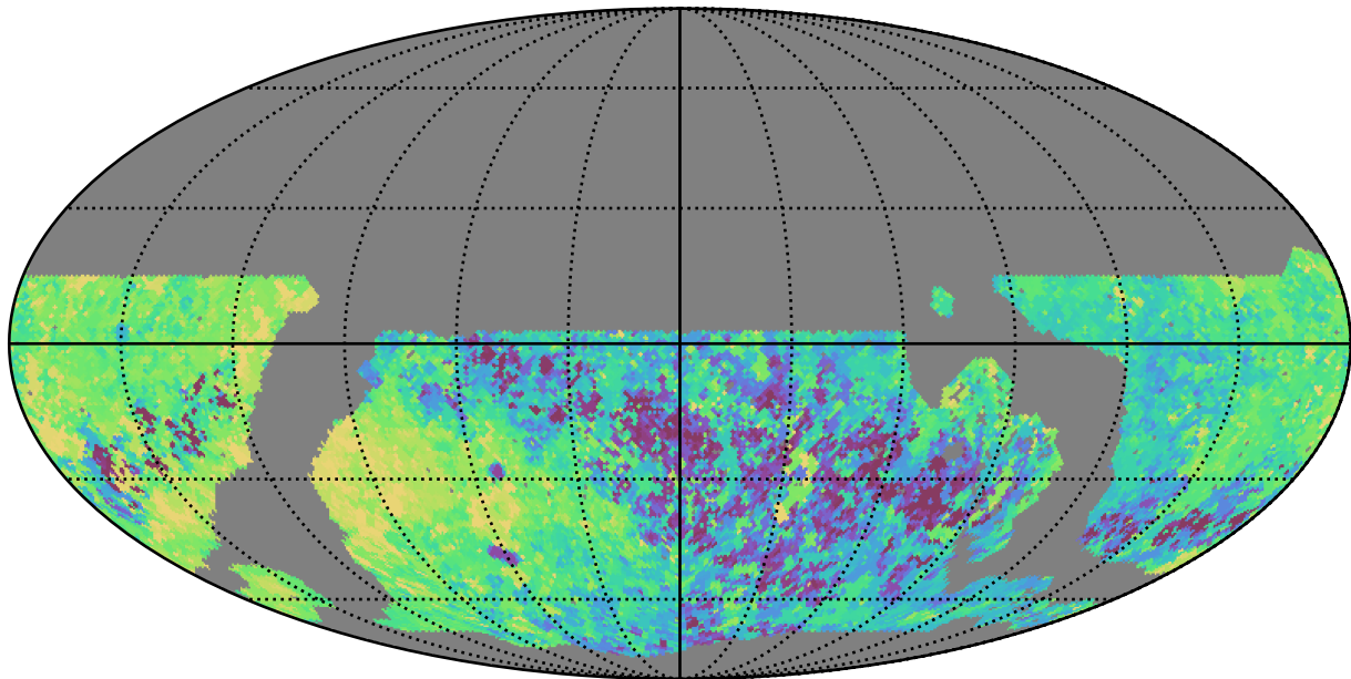
noroll_mjdp60_v3.4_10yrs WFD all bands: Max Inter-Night Gap
