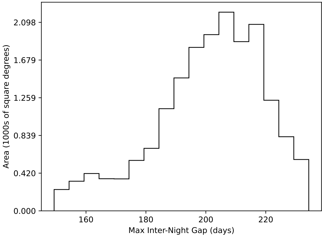
noroll_mjdp60_v3.4_10yrs WFD all bands: Max Inter-Night Gap
