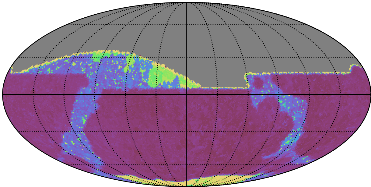
noroll_mjdp60_v3.4_10yrs All sky z band: Max Inter-Night Gap
