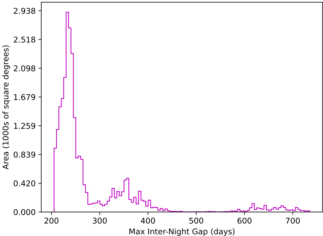
noroll_mjdp60_v3.4_10yrs All sky z band: Max Inter-Night Gap
