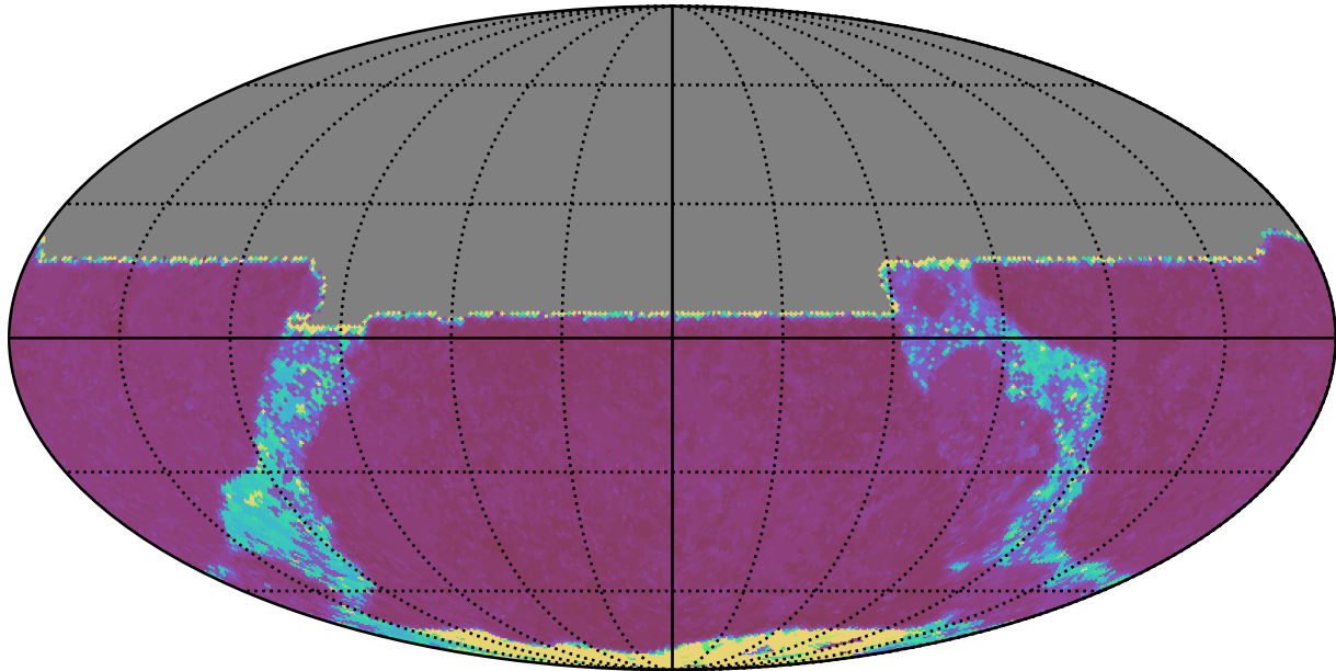
noroll_mjdp60_v3.4_10yrs All sky y band: Max Inter-Night Gap
