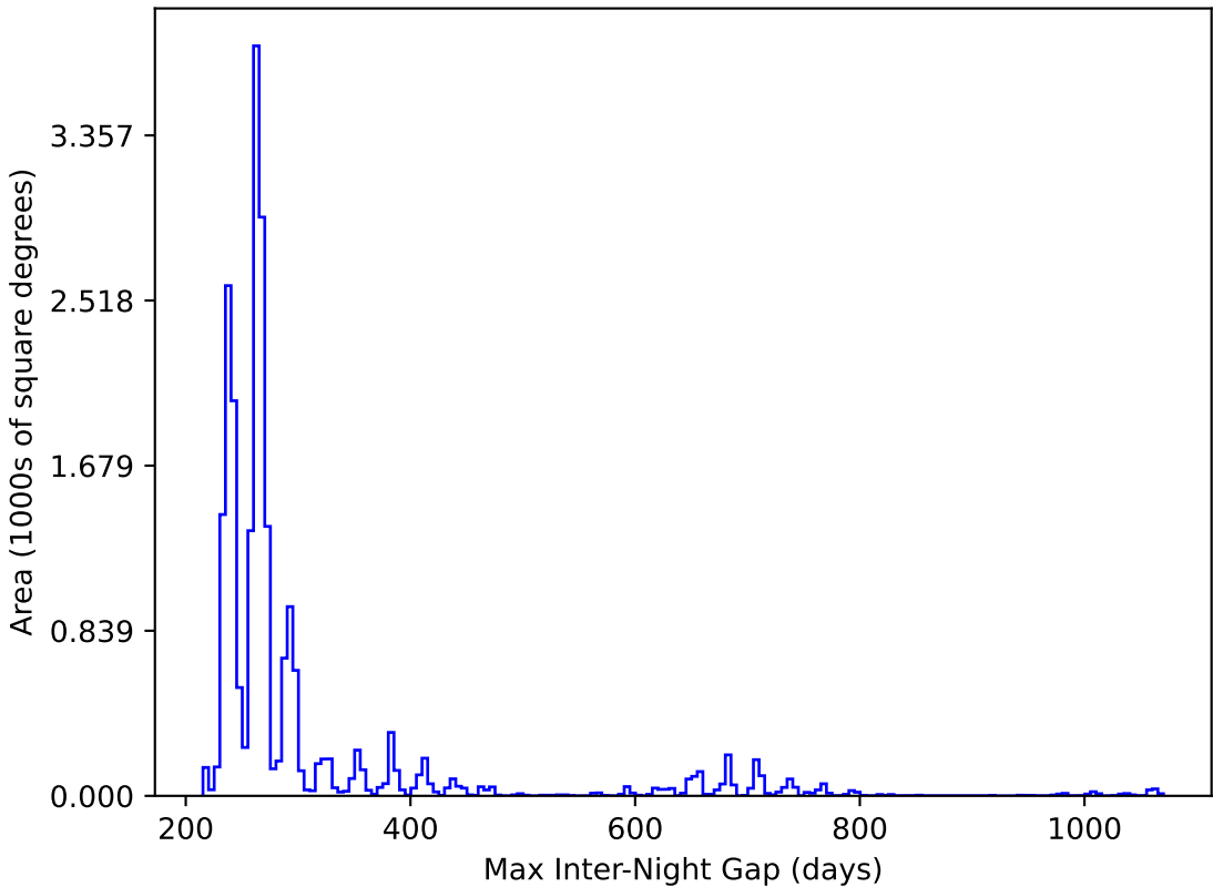
noroll_mjdp60_v3.4_10yrs All sky y band: Max Inter-Night Gap
