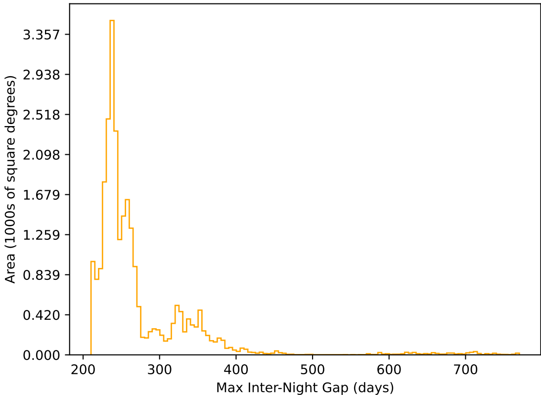
noroll_mjdp60_v3.4_10yrs All sky r band: Max Inter-Night Gap
