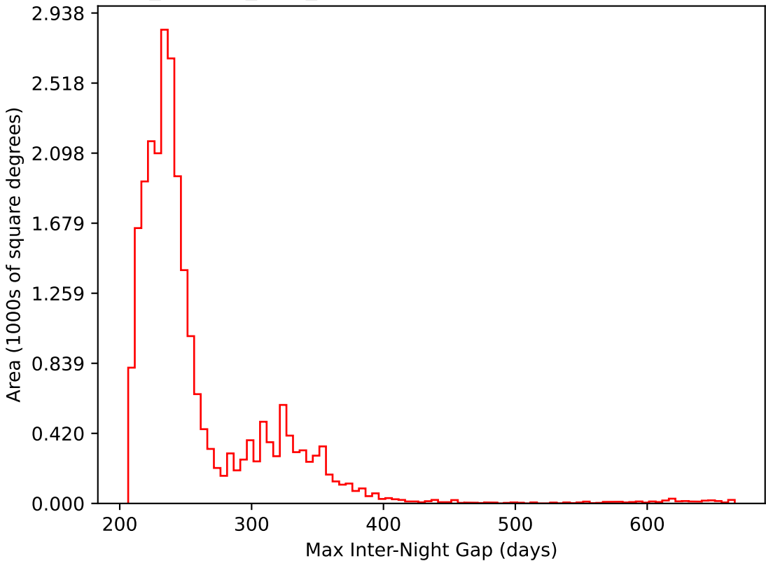
noroll_mjdp60_v3.4_10yrs All sky i band: Max Inter-Night Gap
