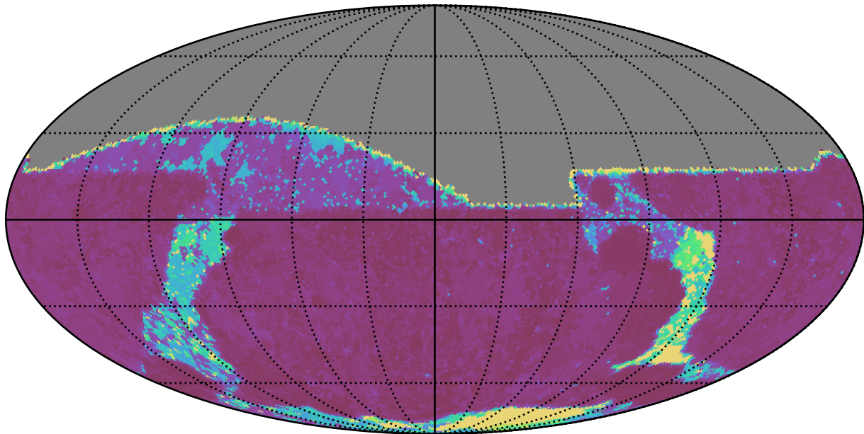
noroll_mjdp60_v3.4_10yrs All sky g band: Max Inter-Night Gap
